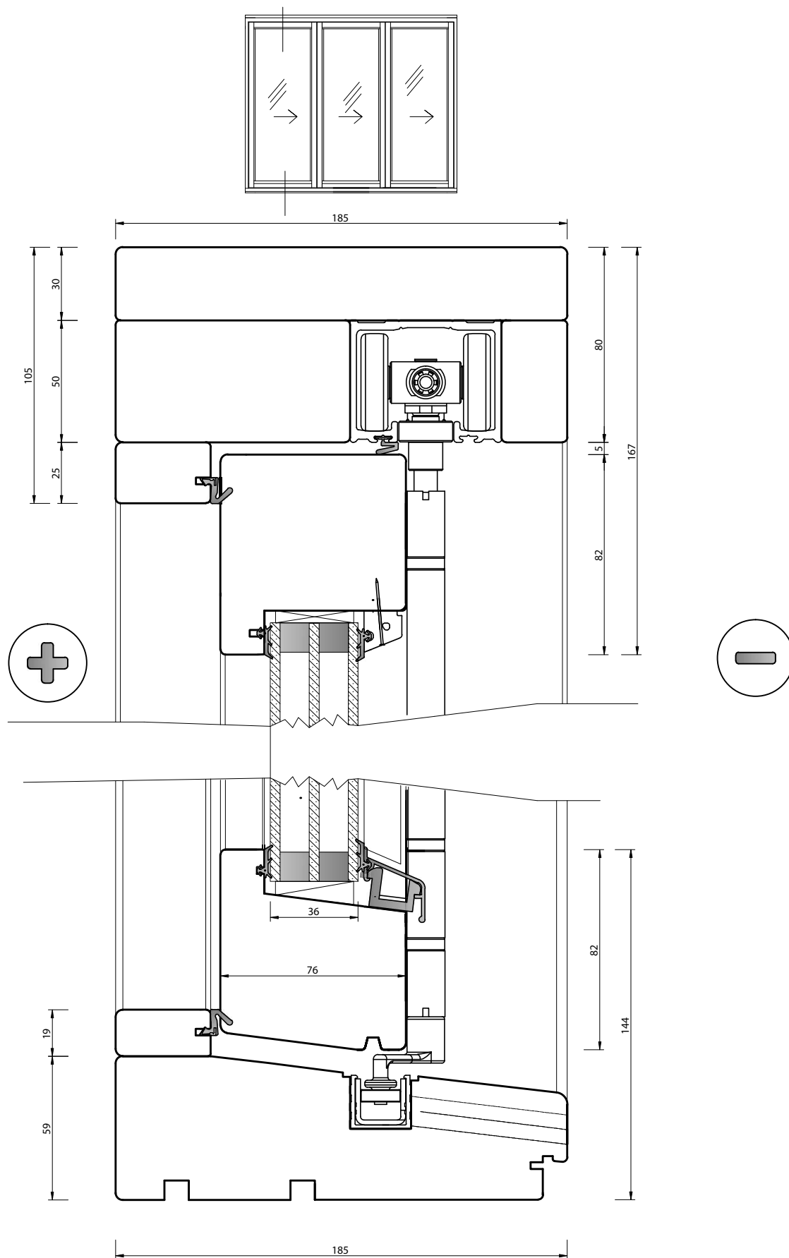
Folding Centor 185/76 Opens outward
