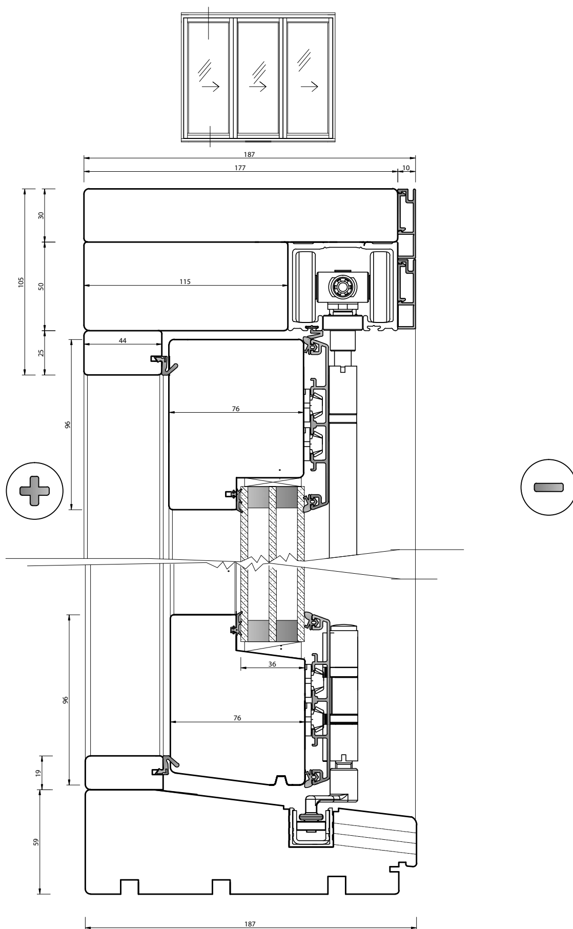
Folding Centor 177/76 Alu clad Opens outward
